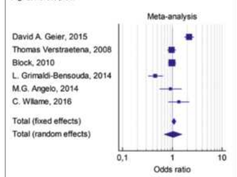
Fig. 2. Forest plot.
